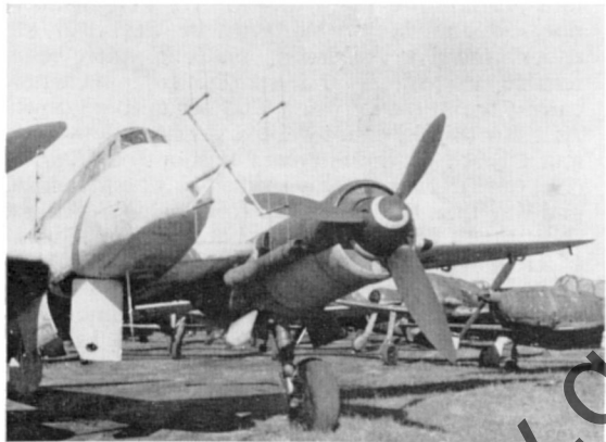
Ju 88G-7b fitted with FuG 218 Neptun radar and FuG 101 Hirschgeweih aerial array. The elements were shorter than those used with SN-2, measuring only 90 cm. Note the belly entrance/escape hatch.
